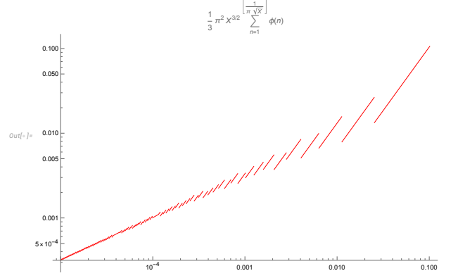
Figure 22. The log-log-plot of the distribution f_X(X) . It is equals \frac{\pi^3}{3} \Phi(k) X \sqrt{X} at each internal \frac{1}{\pi^2(k+1)^2} < X < \frac{1}{\pi^2 k^2} with positive integer k . Asymptotically f_X(X) \rightarrow \frac{\pi\sqrt{X}}{3} at X \rightarrow 0 .
