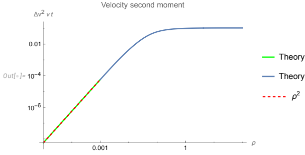
Figure 19. The universal function (95) as a function of \rho = |\vec{r}|/\sqrt{\bar{v}t} . The turnover is caused by subleading terms in the power expansion starting with \rho^2 . The next terms involve quantum oscillations manifesting as a turnover from power growth to power decay. Asymptotic at large \rho is const as it follows from the table (97) of the decay indexes.
