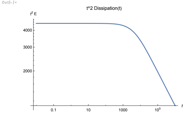
Figure 29. The log-log plot energy dissipation t^2\mathcal{E}(t) as a function of t has a regime change due to quantum effects. It starts as constant at small t and asymptotically decays as t^2\mathcal{E} \propto t^{-1/4} .
