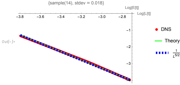
Figure 12. The log-log plot of the decaying energy as a function of decaying length scale L(t) . Red dots are the DNS data, the green curve is an exact theoretical curve, and the dashed blue line is its asymptotic limit E(t) \propto L(t)^{-5/2} corresponding to E \propto t^{-5/4} .
